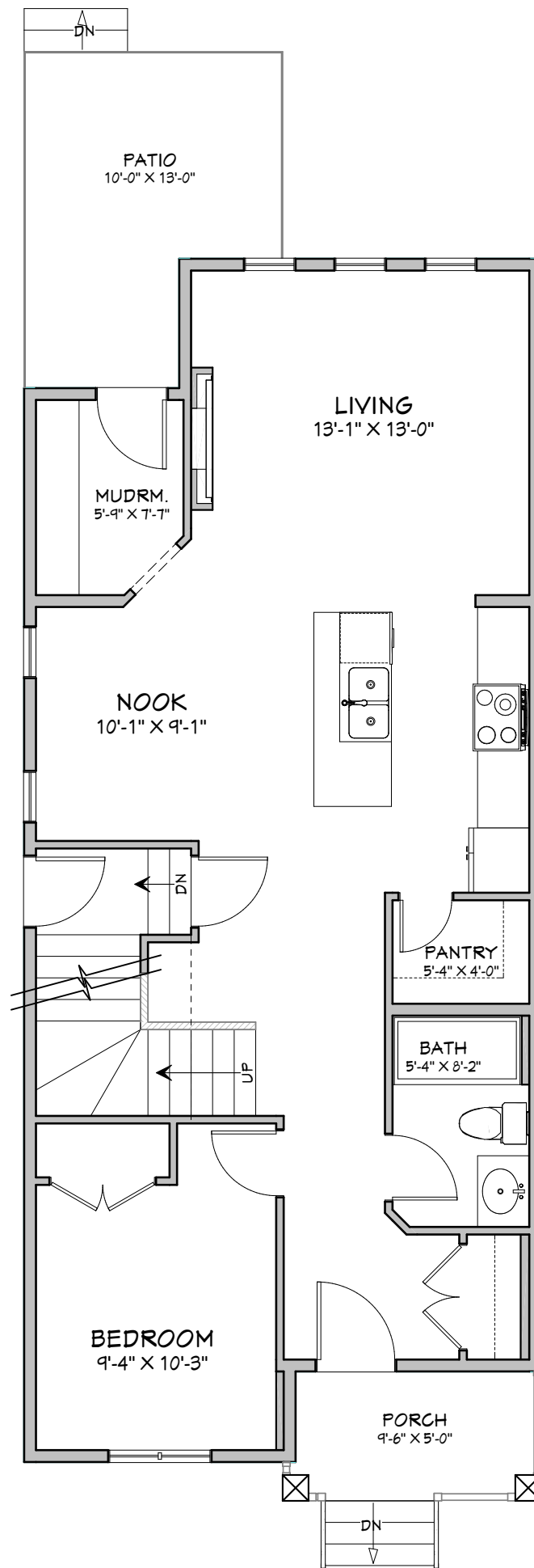
MAIN FLOOR 867 SQ.FT.
