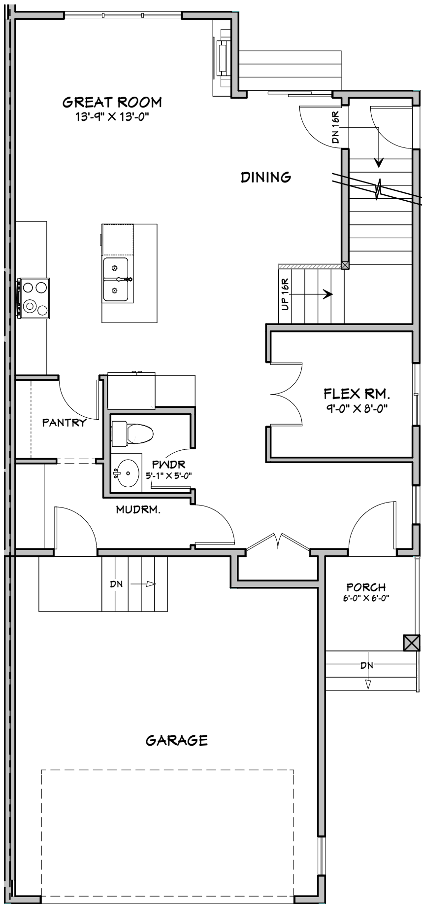
MAIN FLOOR 852 SQ.FT.
