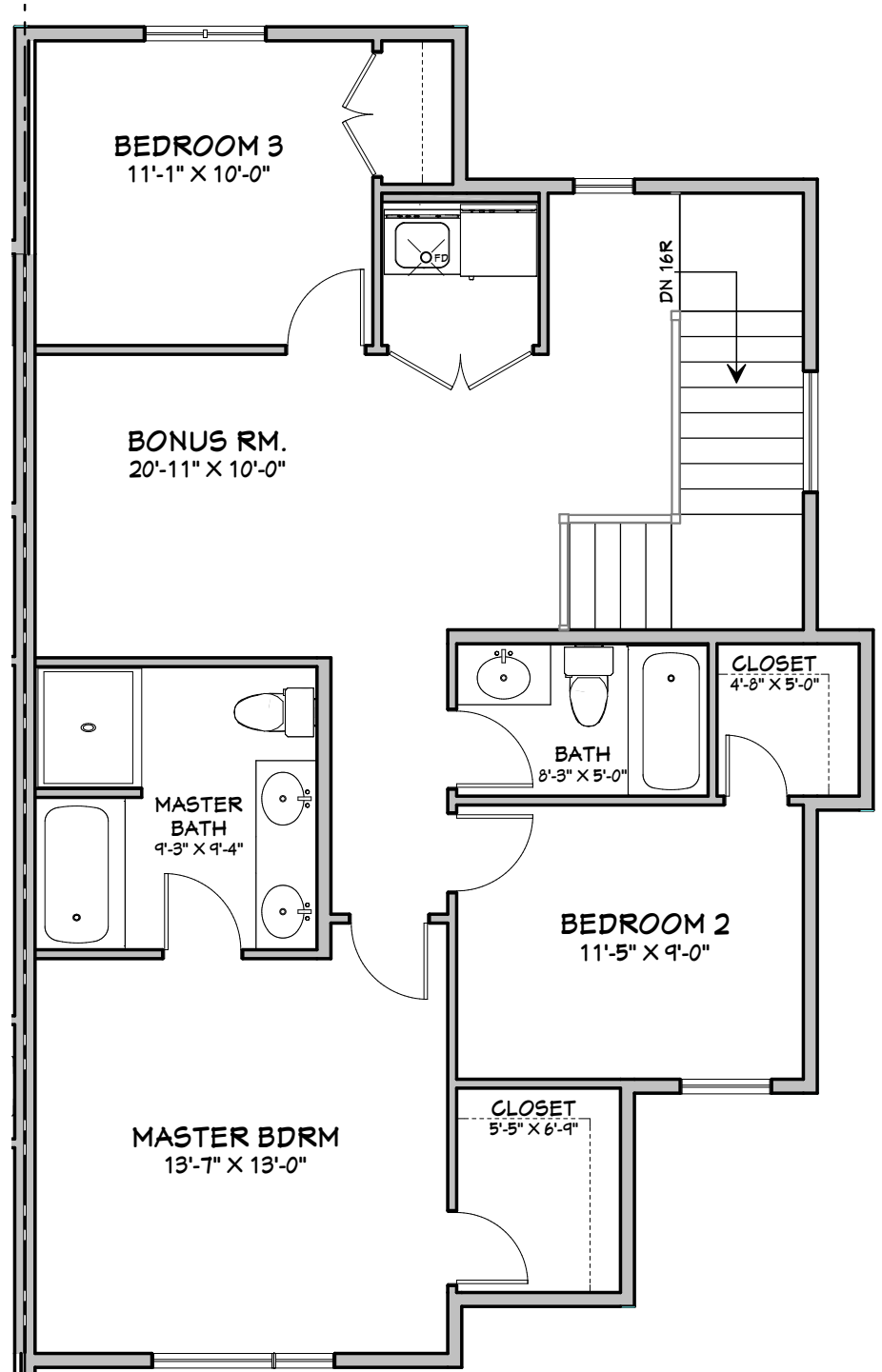
SECOND FLOOR 952 SQ.FT.
