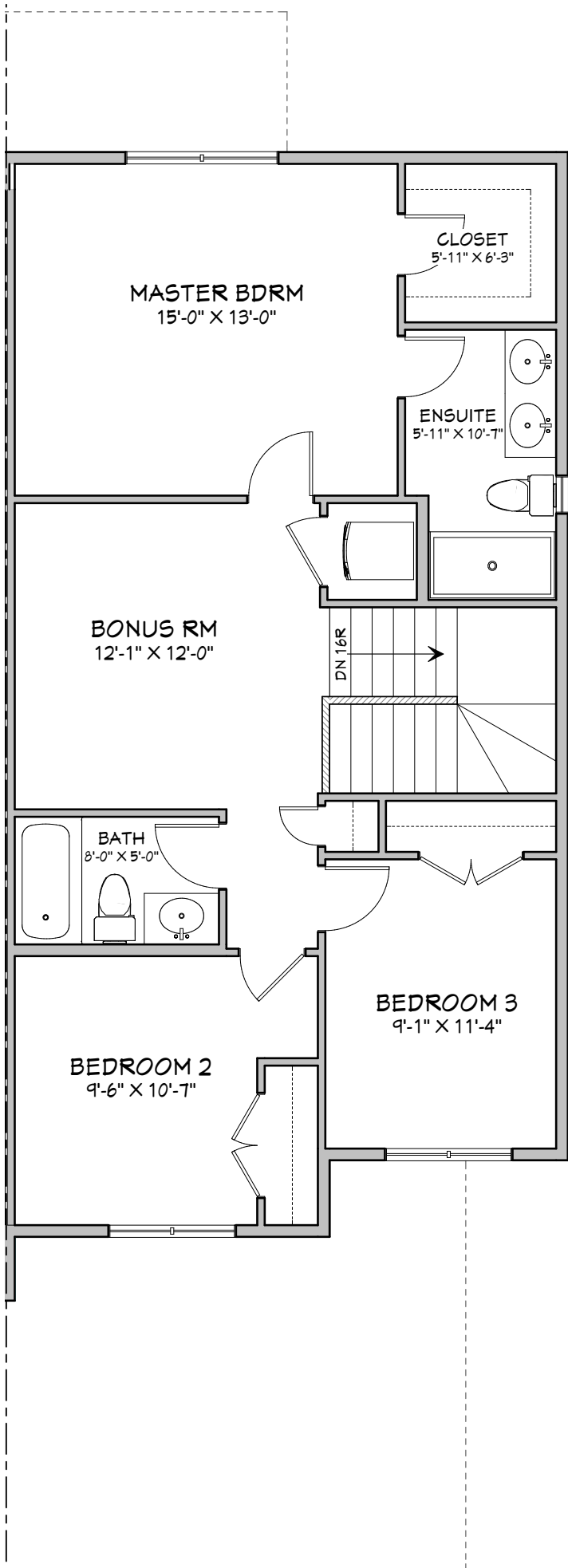
SECOND FLOOR 839 SQ.FT.
