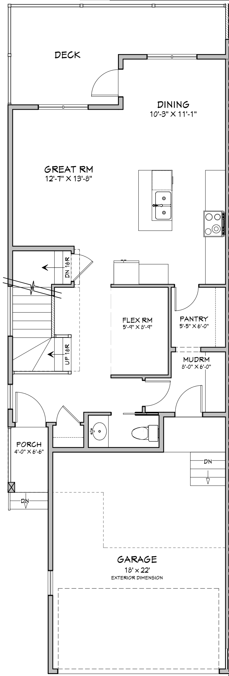
MAIN FLOOR 781 SQ.FT.
