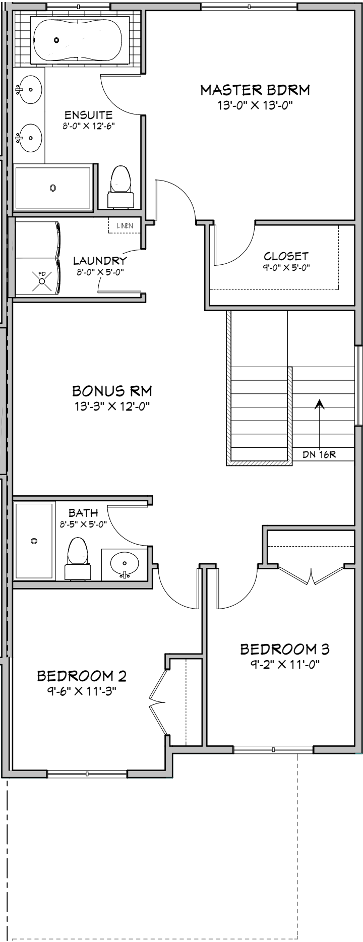
SECOND FLOOR 963 SQ.FT.
