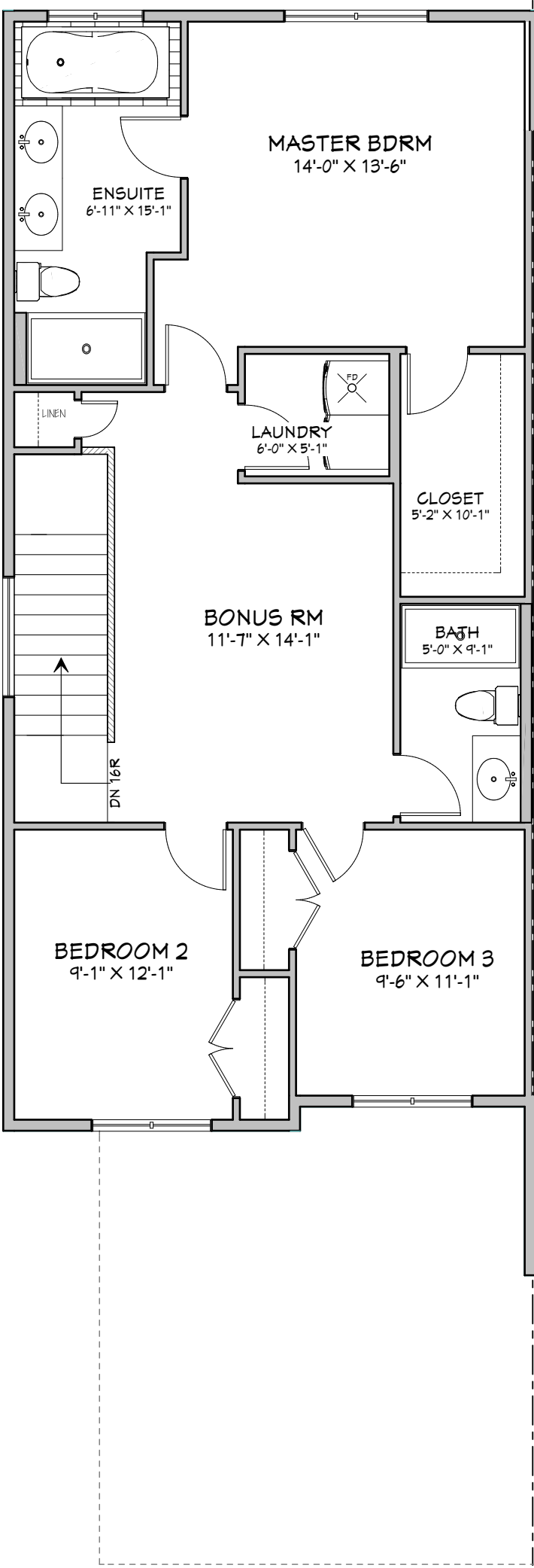
SECOND FLOOR 947 SQ.FT.
